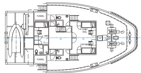
FORECASTLE DECK PLAN
