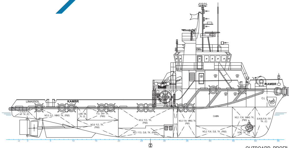
OUTBOARD PROFILE
